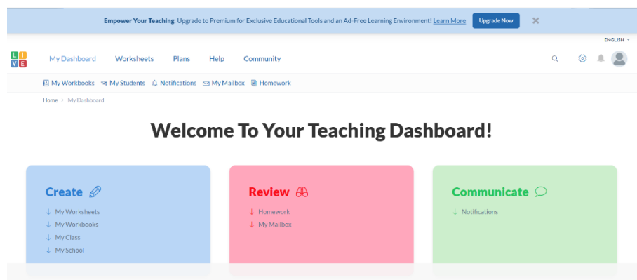
Figure 4. Creat sheet
