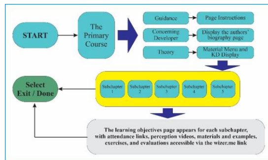
Figure 34. Flowchart of media structure
